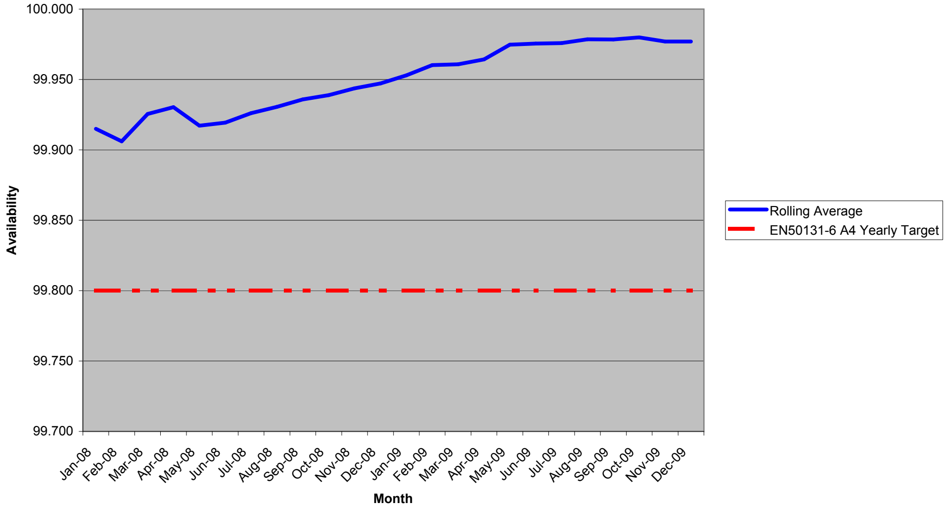
UK-0 Measured Availability - Rolling 12 months
