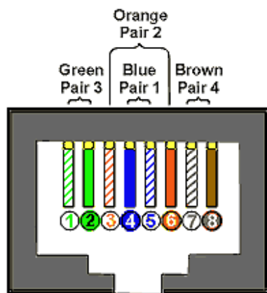
RJ-45 JACK TIA/EIA 568A STANDARD
