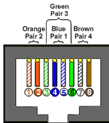
RJ-45 JACK TIA/EIA 568B STANDARD
